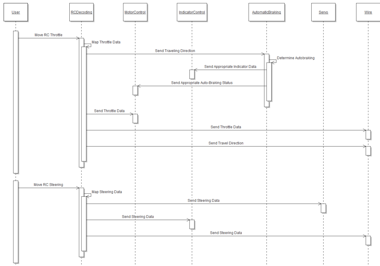
Figure 4. Sequence Diagram for the Control System's RC Mode.
