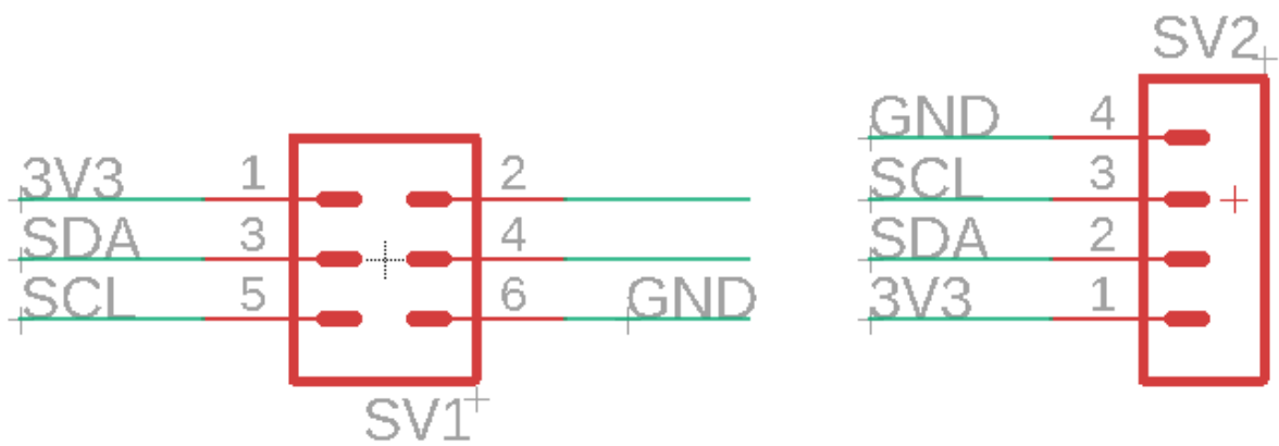
Figure 87. Jetson Nano I2C Breakout Board Schematic.
