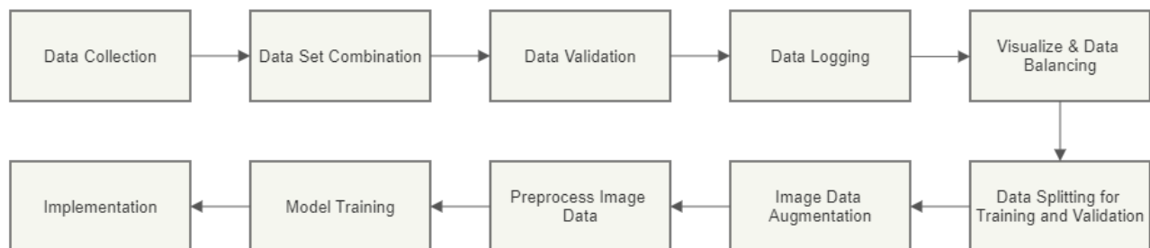
Figure 92. A.I. Training Diagram.
