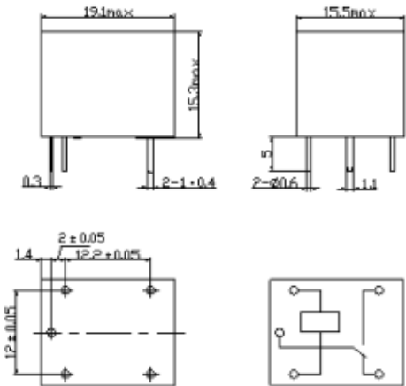
Figure 35. Songle SRD-12VDC-SL-C Relay Datasheet Page 1 of 2.
