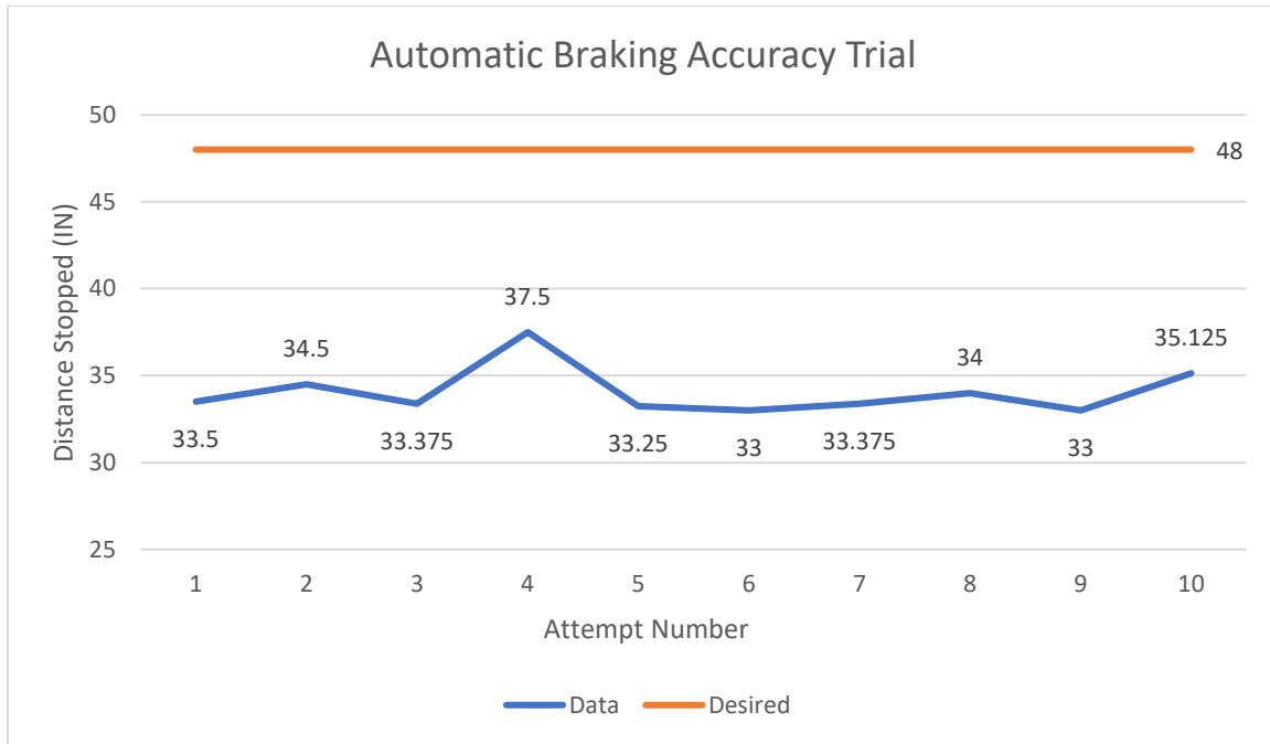
Figure 3. Automatic Braking Accuracy Trial Result Graph.
