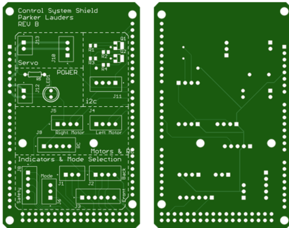
Figure 82. Control System Arduino Mega 2560 REV 3 Shield Board.
