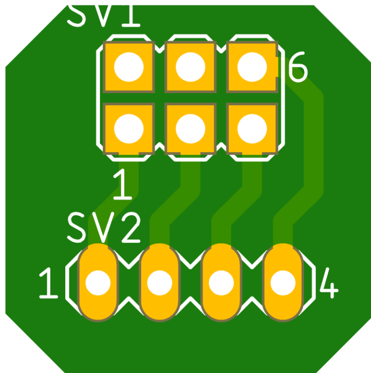
Figure 88. Jetson Nano I2C Breakout Board.
