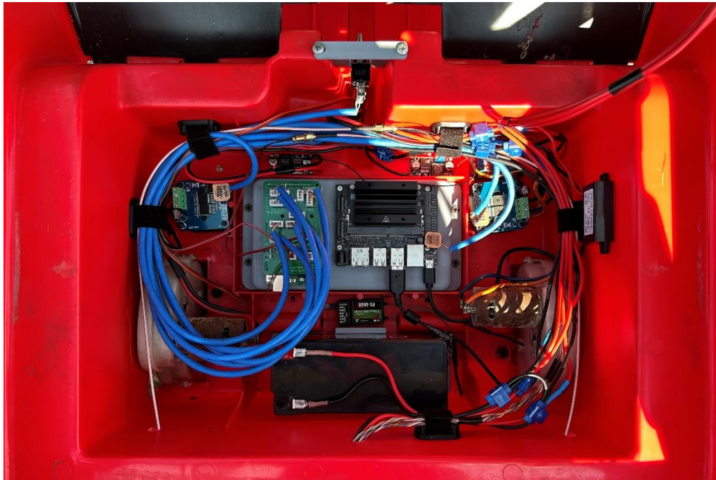
Figure 101. Completed Electronic Bay.
