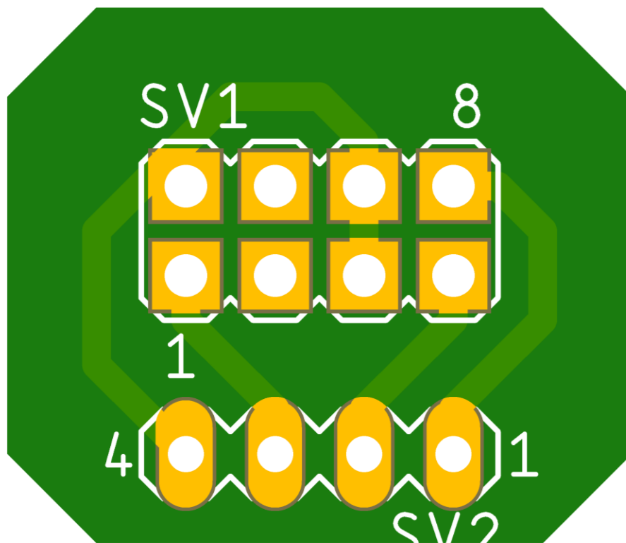
Figure 85. Motor Controller Breakout Board Schematic.
