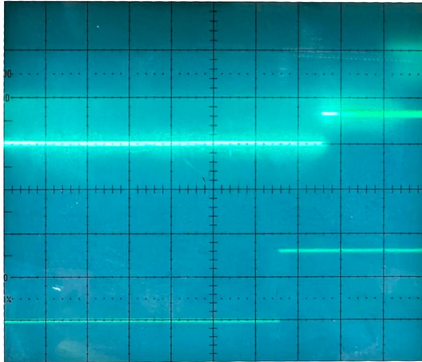
Figure 99. RC PWM Signal for Right/Forward RC Signals (Bottom Signal).
