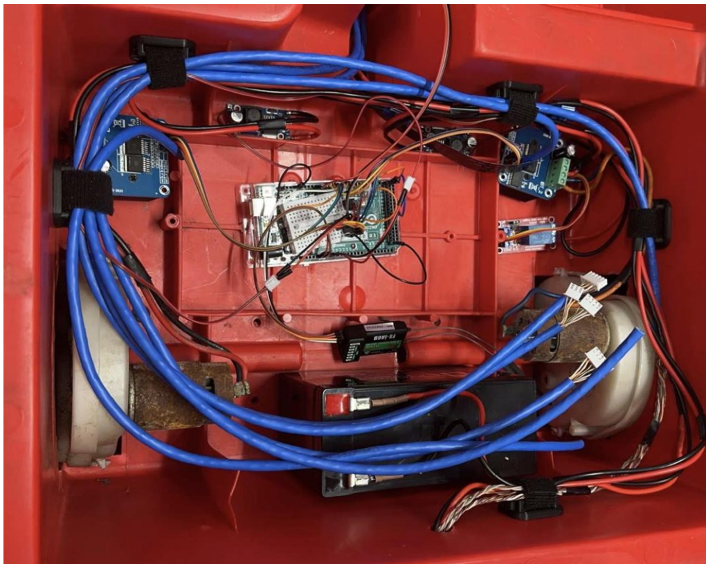
Figure 100. BTS7960 Motor Controller Integration Prototyping.
