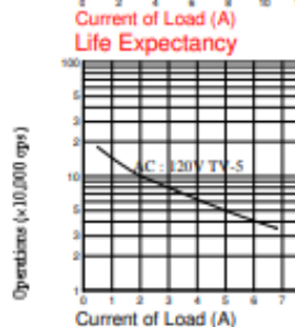
Figure 36. Songle SRD-12VDC-SL-C Relay Datasheet Page 2 of 2.
