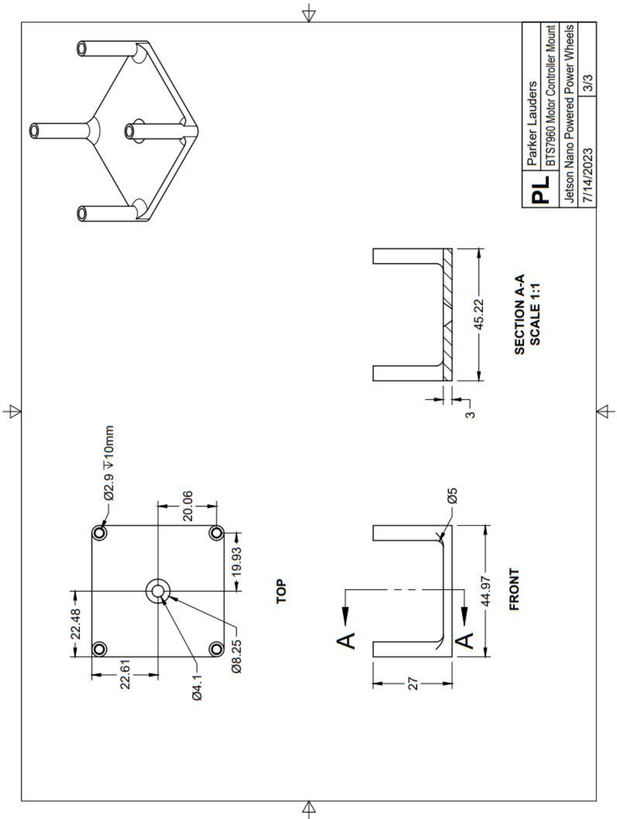
Figure 59. BTS7960 Motor Controller Mount Drawing File Page 3 of 3.
