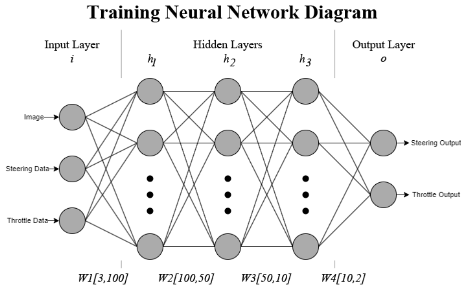
Figure 8. Training CNN Neural Network Diagram.
