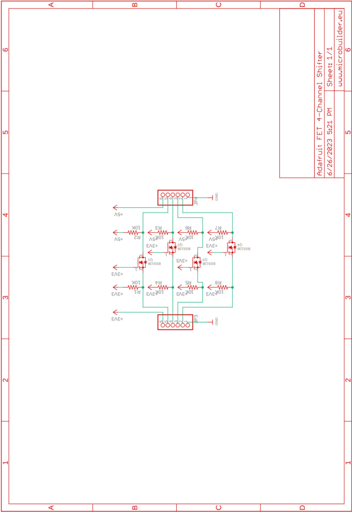
Figure 81. Adafruit 4-Channel Level Shifter Schematic.
