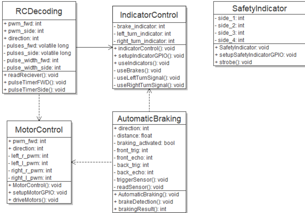
Figure 90. Control System Class Diagram.
