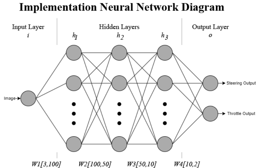
Figure 9. Implementation CNN Neural Network Diagram.
