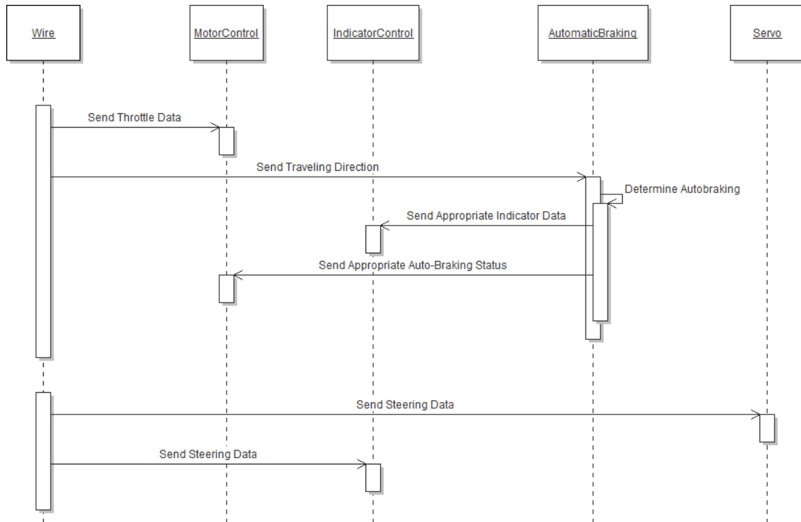
Figure 2. Sequence Diagram for the Control System When in A.I. Mode.
